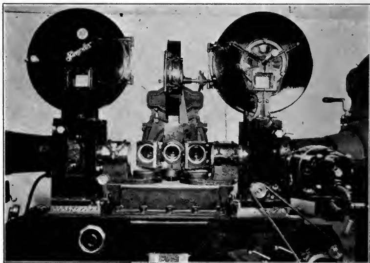
FIG. 4. Front close-up view, showing lens mounts, mirror holders, and optical bench. The Bell & Howell camera movement can be seen through the window in the left-hand head; sync motor on right-hand head.
